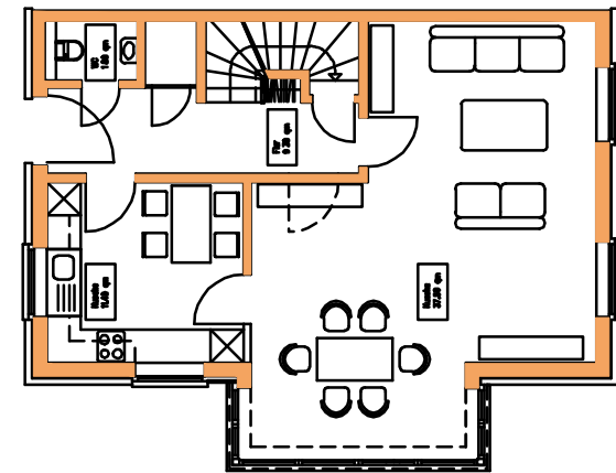
ALTERNATIVE GLASERKER GRUNDRISS
